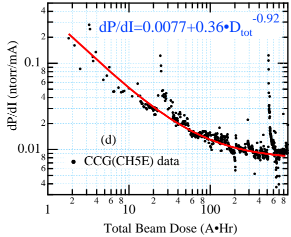
Figure 7. The beam induced dynamic pressure rise, ( dP/dI ), at various locations in the IR. (a) The dynamic pressure rise at Q1E; (b) a similar plot for a gauge on the beamline next to the ISP chambers, and (c) for the soft-bend chambers. (d) shows a similar plot for a gauge within the hard-bend sector pumped only by distributed ion pumps (DIPs), but where the SR flux and gas load is the most intense.
