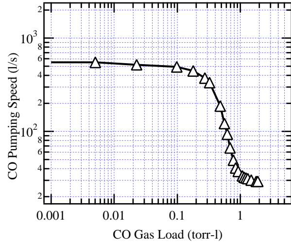
Figure 5. Pumping Speed in the Q1 TiSP chamber.
