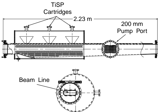
Figure 2. The ISP Chamber with Ti pumping plenum.
