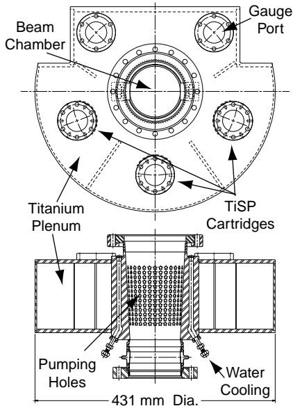
Figure 1. The Q1 titanium pump chamber. Above, view along beam. Below, cross-section looking down.
