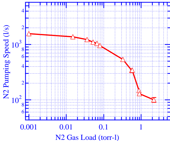
Figure 4. N 2 Pumping Speed, Soft-Bend Chamber.
