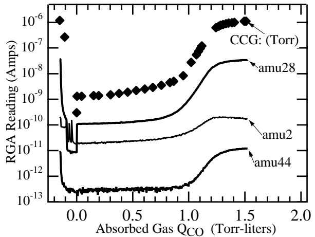
Figure 6. Saturation of the ISP chamber with CO gas. The CCG pressure is on the same axis scale, in Torr.
